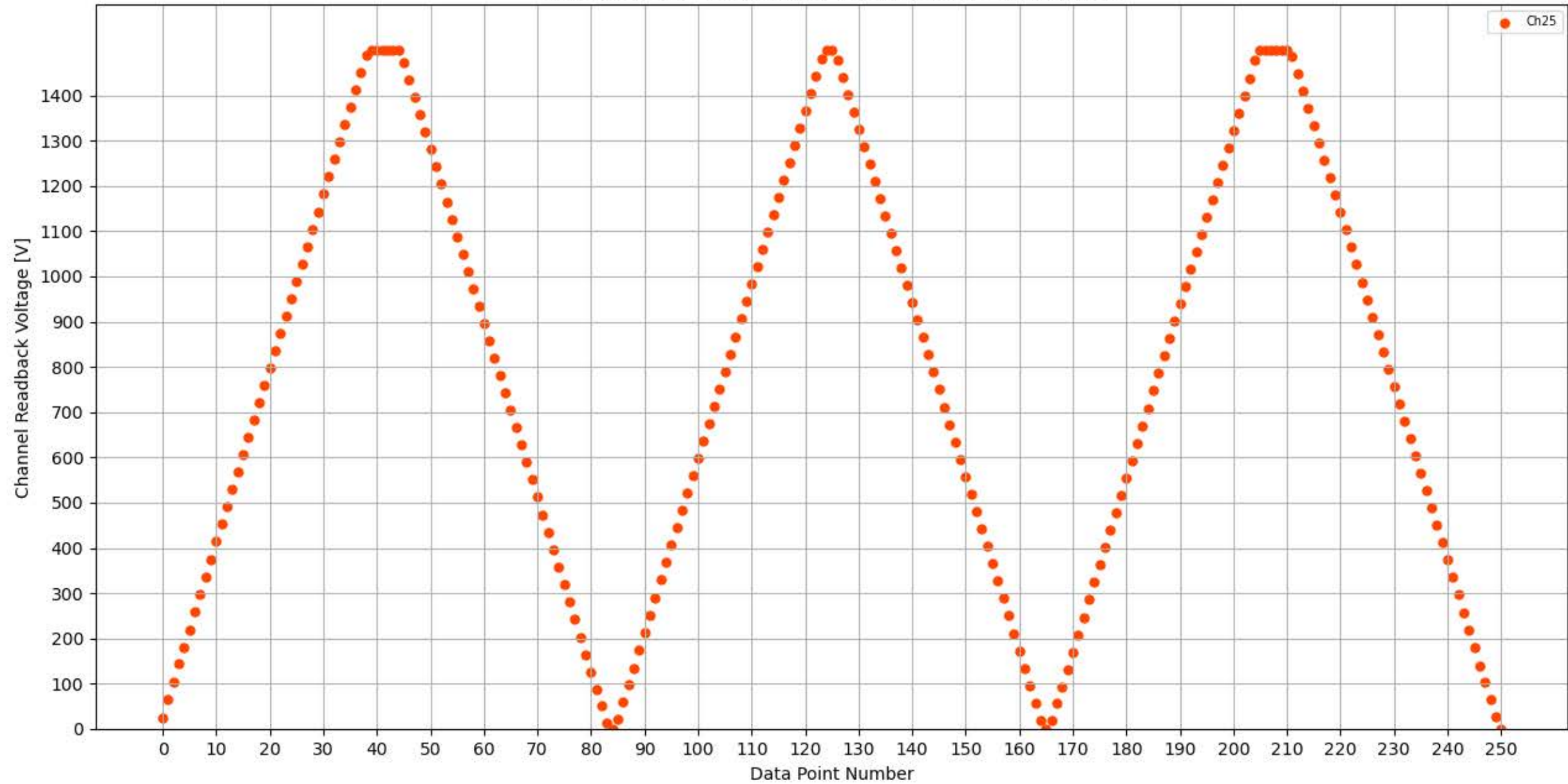
Voltage Ramp Test (Python) Bd #354, Slot #14, Ch #25
