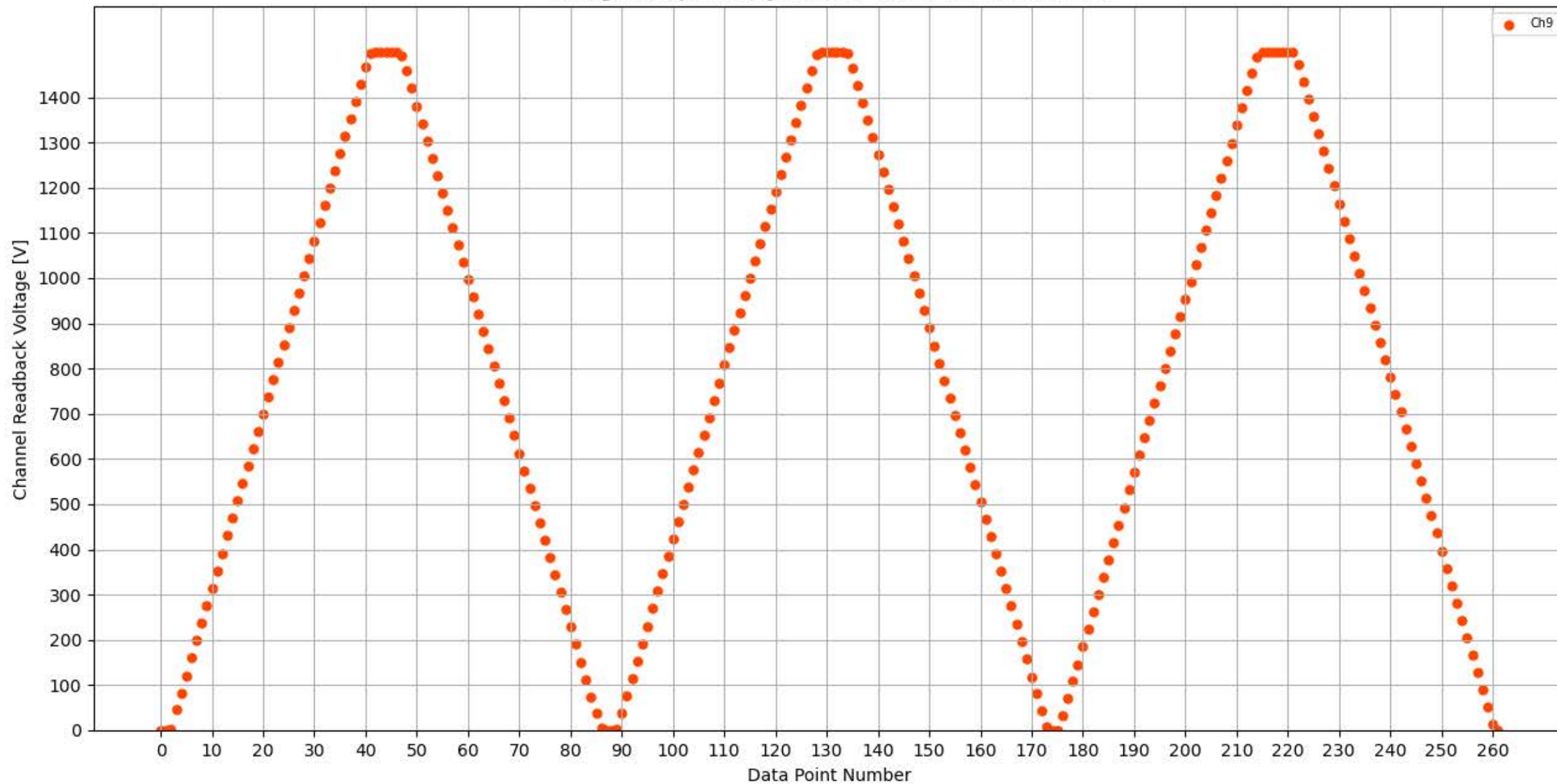
Voltage Ramp Test (Python) Bd #354, Slot #14, Ch #9
