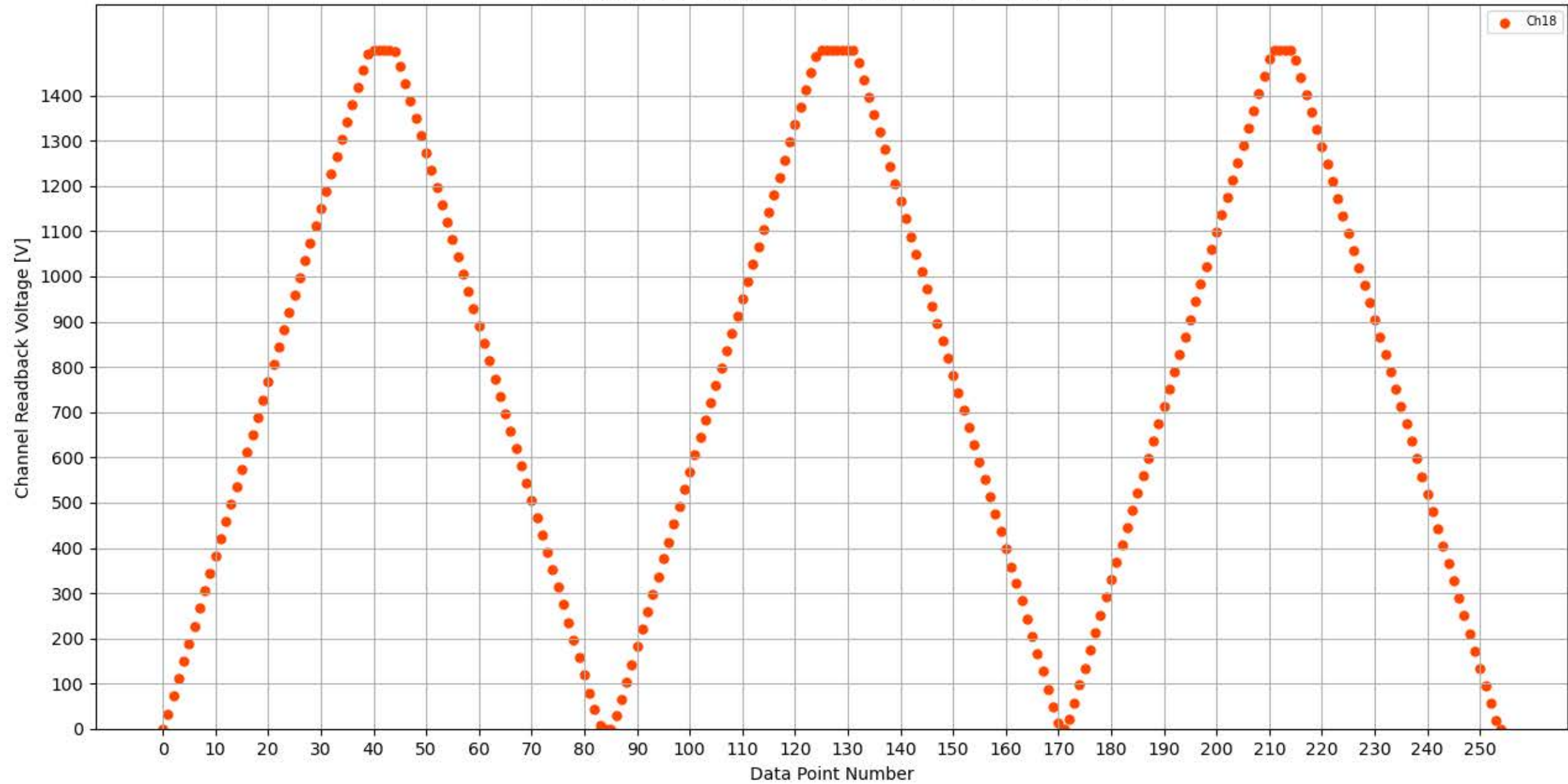
Voltage Ramp Test (Python) Bd #354, Slot #14, Ch #18
