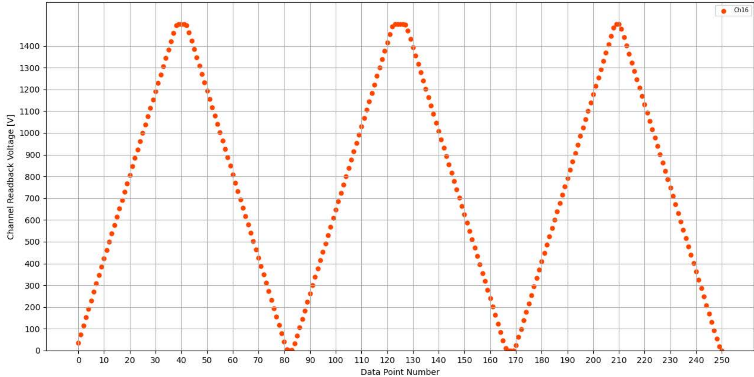
Voltage Ramp Test (Python) Bd #354, Slot #14, Ch #16
