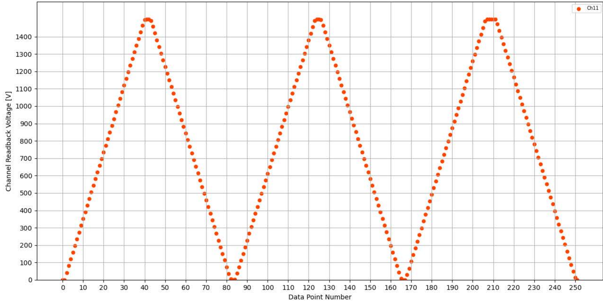
Voltage Ramp Test (Python) Bd #354, Slot #14, Ch #11
