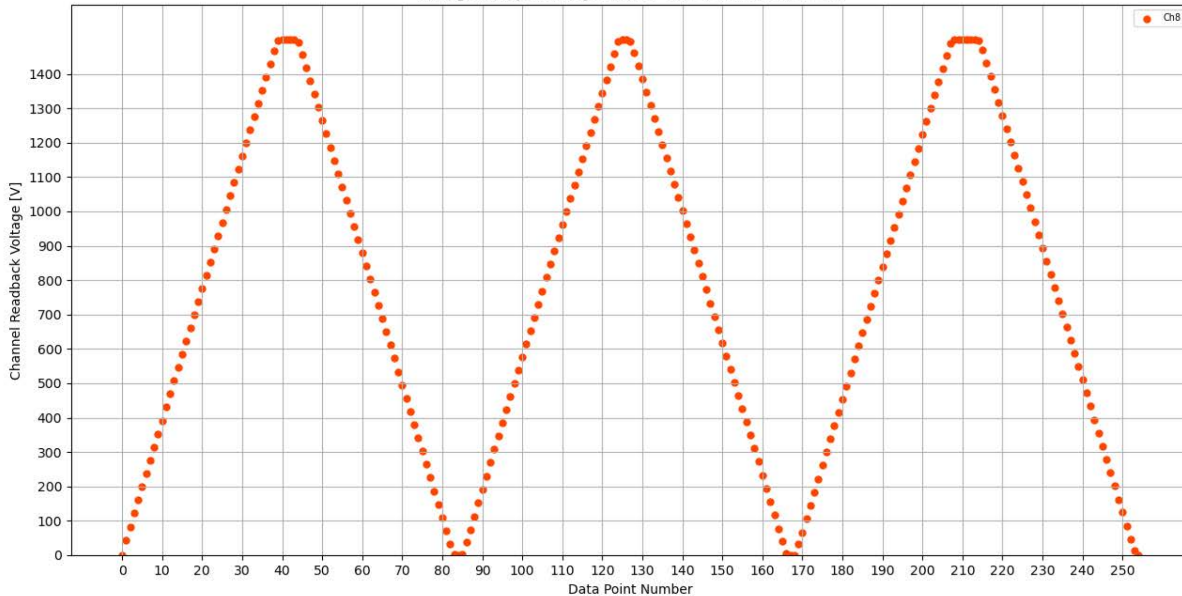
Voltage Ramp Test (Python) Bd #354, Slot #14, Ch #8
