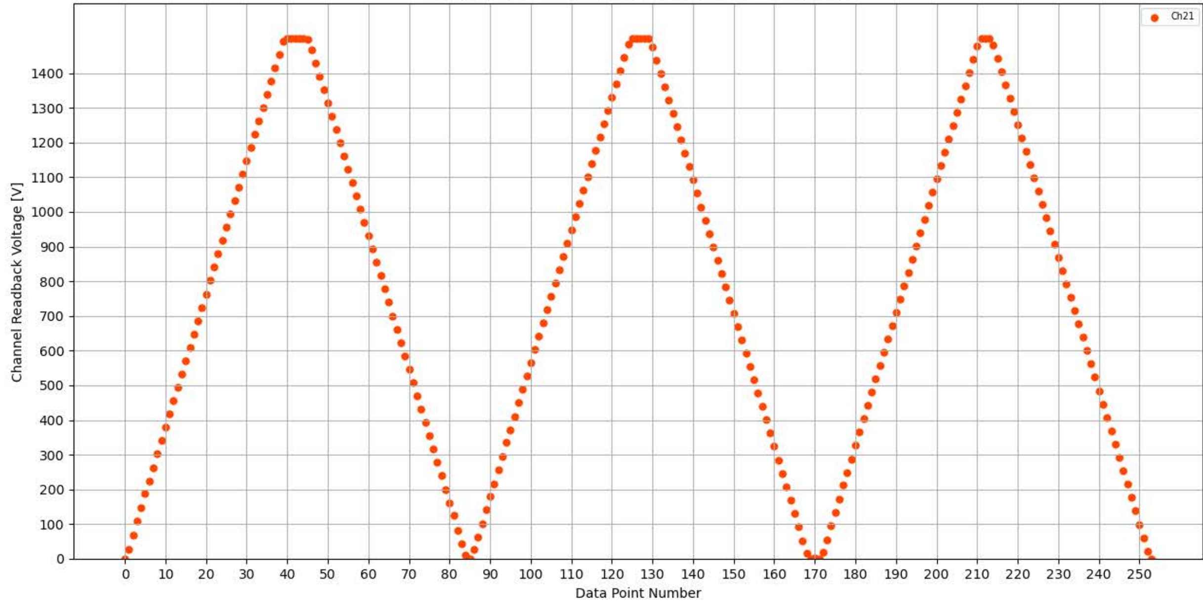
Voltage Ramp Test (Python) Bd #354, Slot #14, Ch #21
