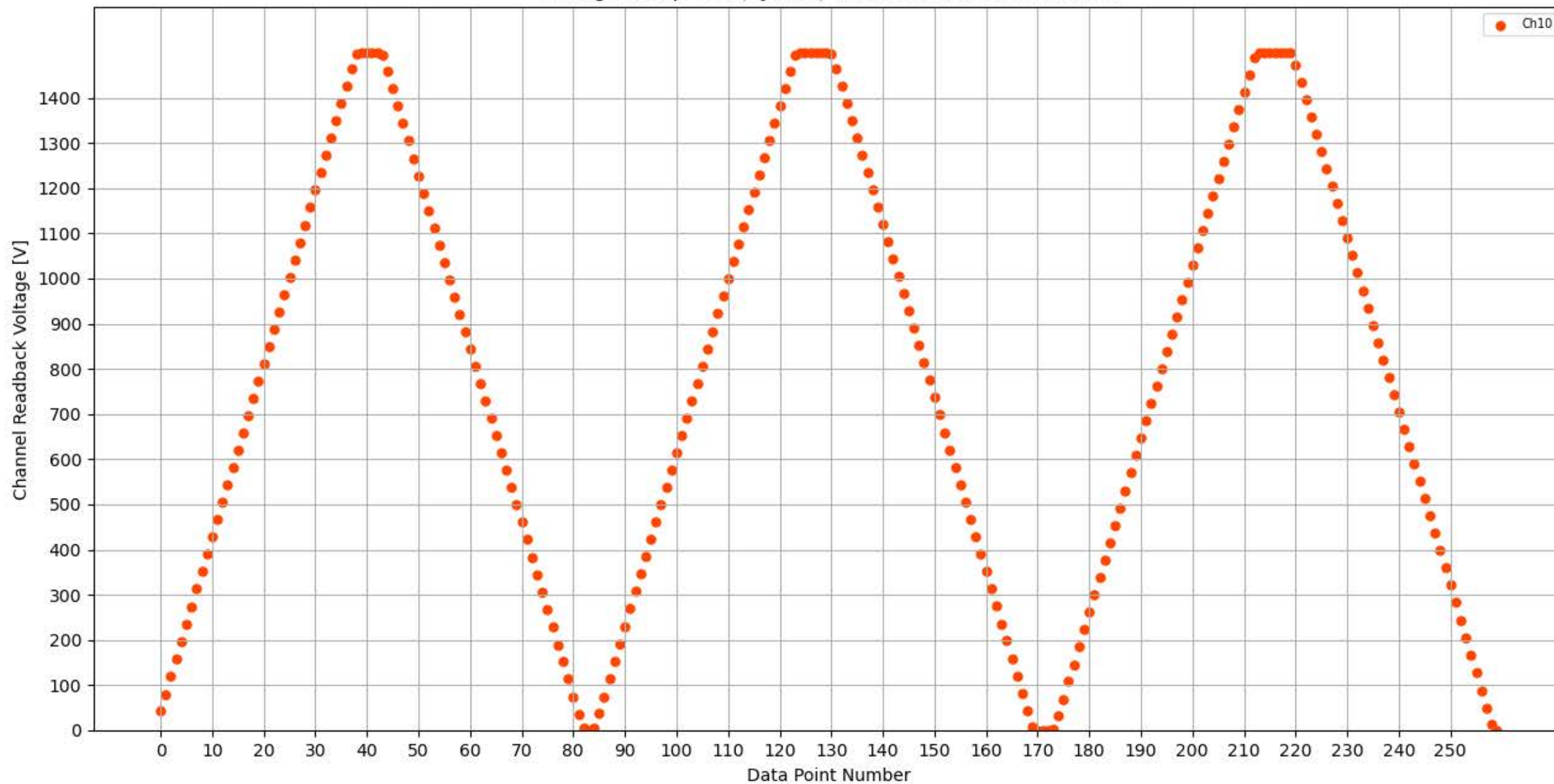
Voltage Ramp Test (Python) Bd #354, Slot #14, Ch #10
