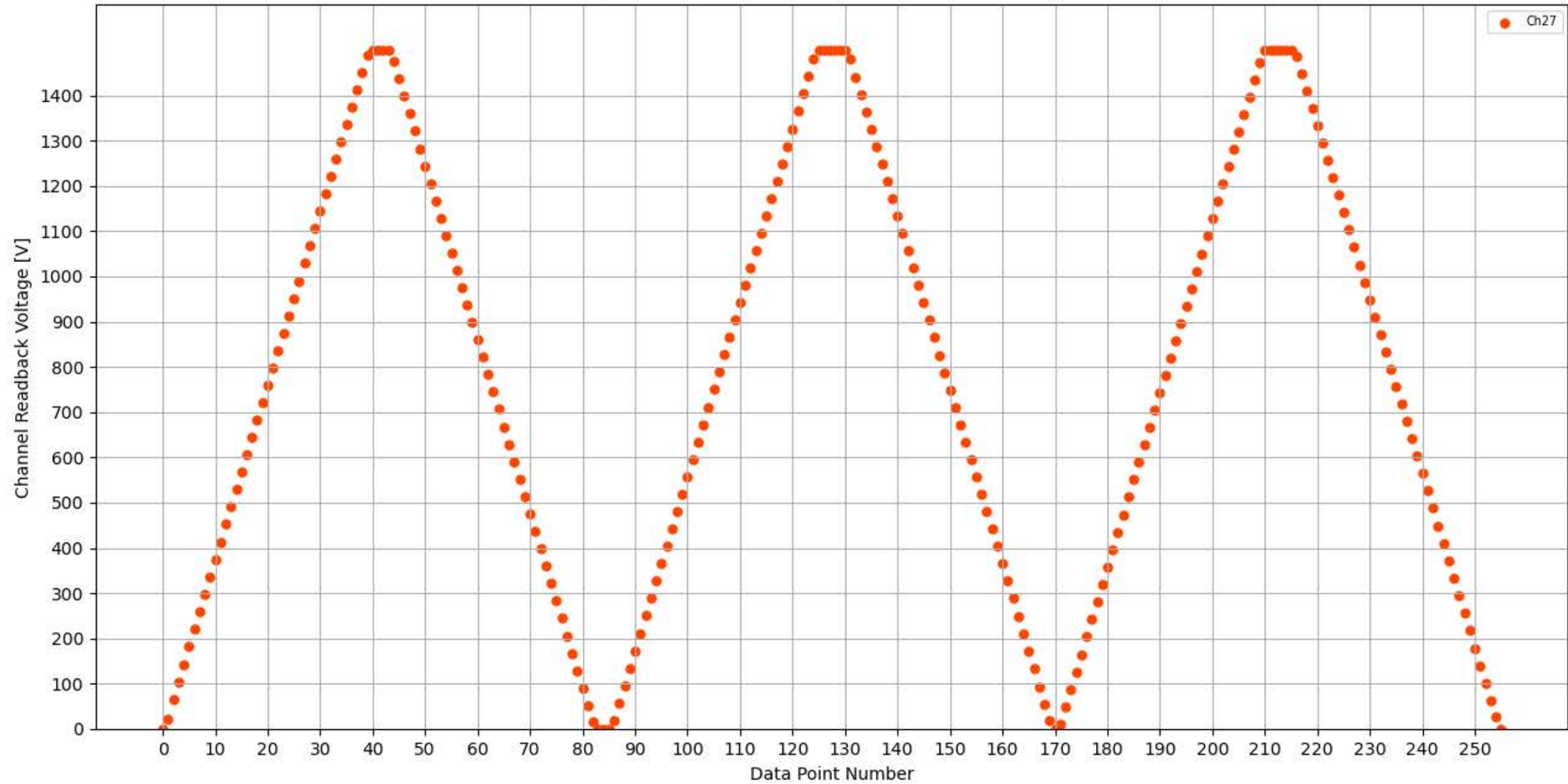
Voltage Ramp Test (Python) Bd #354, Slot #14, Ch #27
