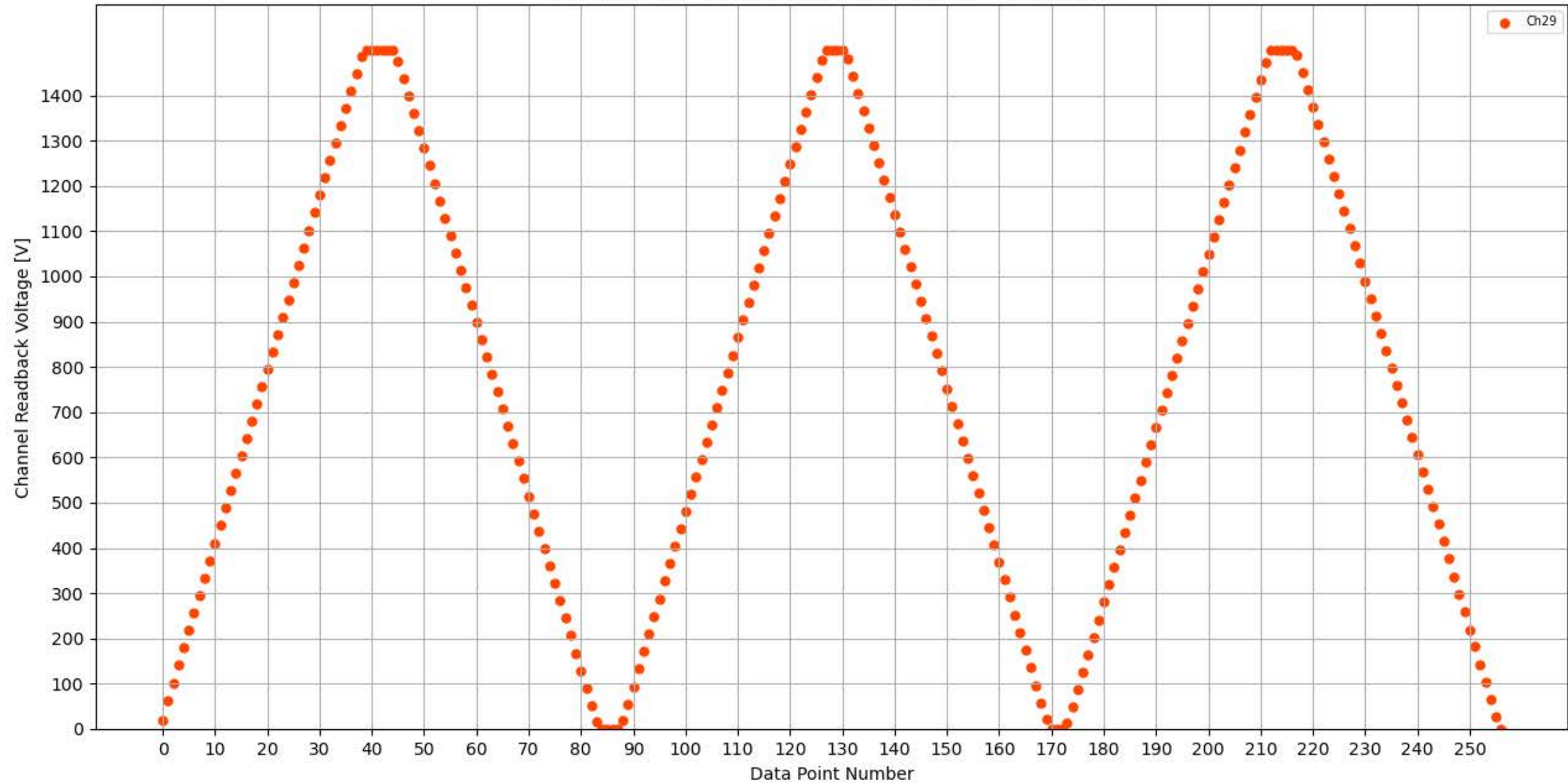
Voltage Ramp Test (Python) Bd #354, Slot #14, Ch #29
