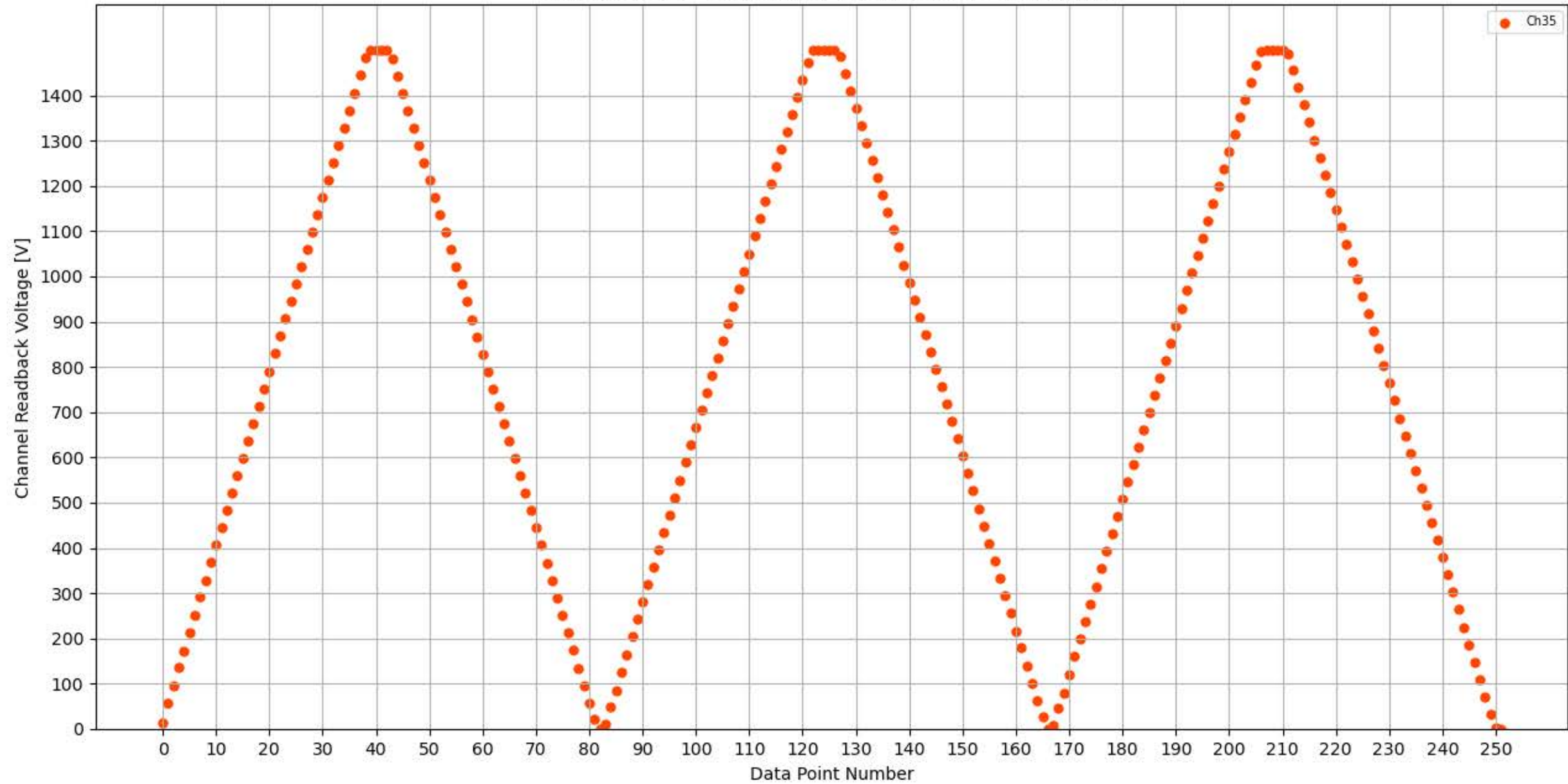
Voltage Ramp Test (Python) Bd #354, Slot #14, Ch #35
