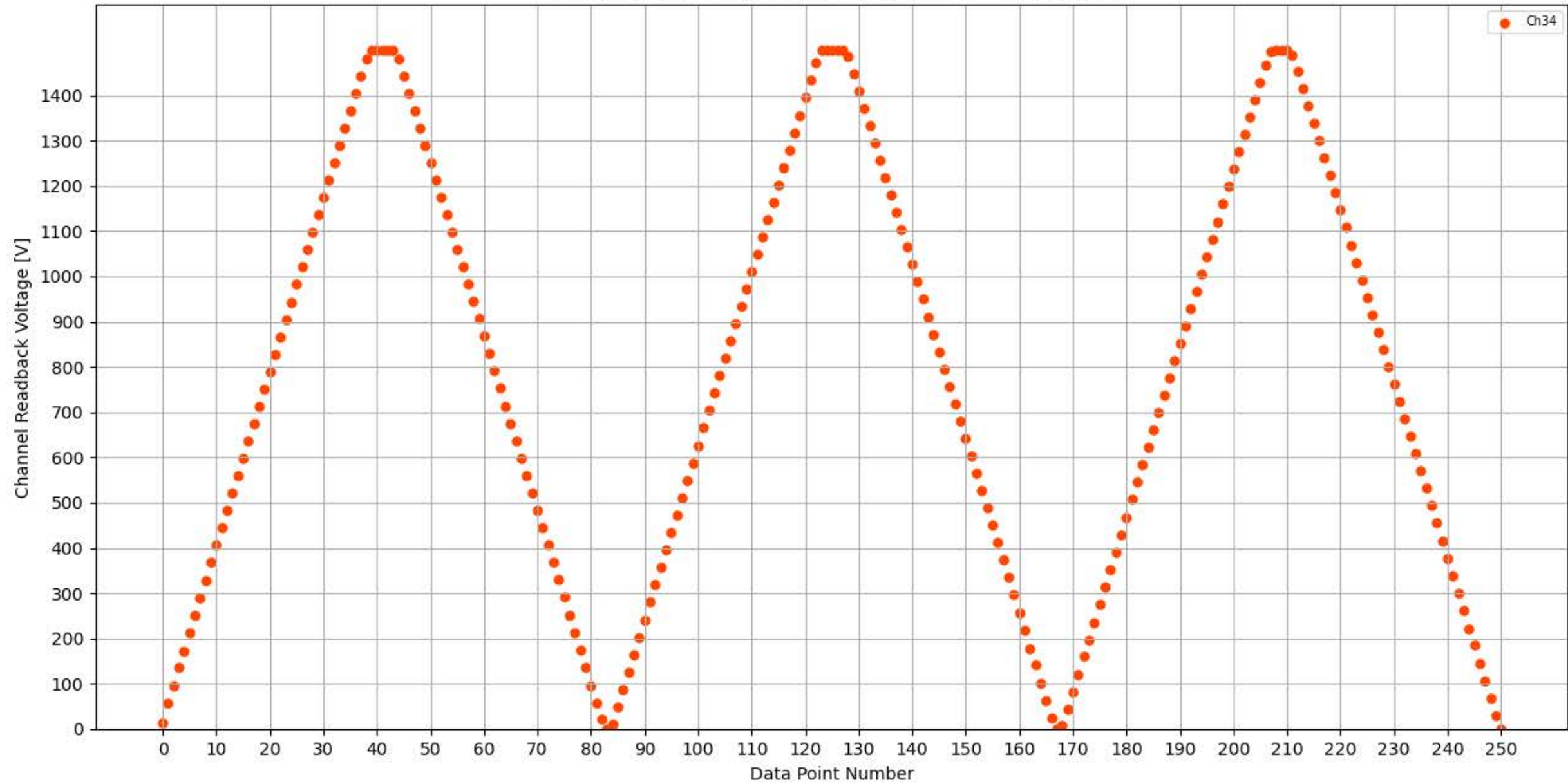
Voltage Ramp Test (Python) Bd #354, Slot #14, Ch #34
