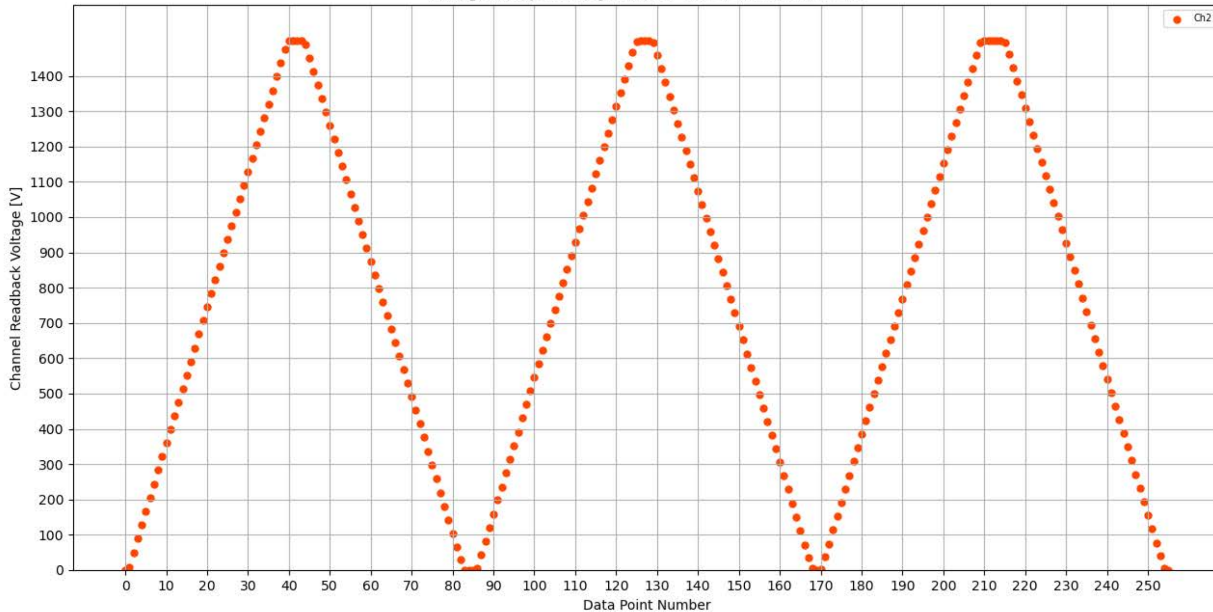
Voltage Ramp Test (Python) Bd #354, Slot #14, Ch #2
