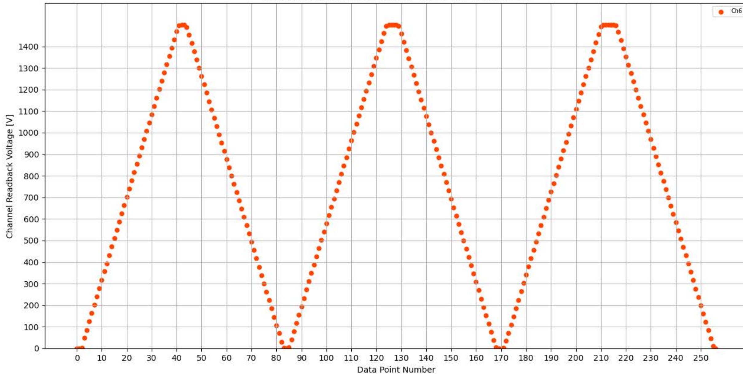
Voltage Ramp Test (Python) Bd #354, Slot #14, Ch #6
