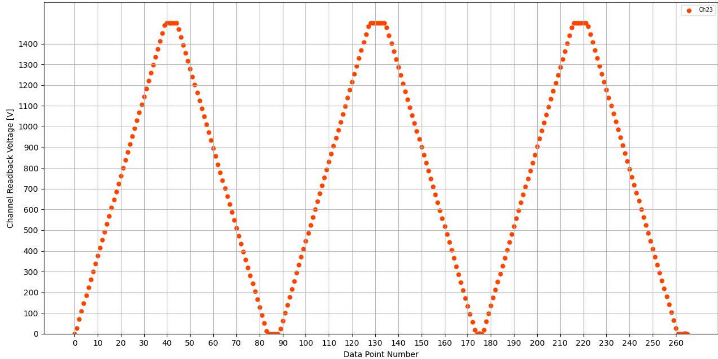
Voltage Ramp Test (Python) Bd #354, Slot #14, Ch #23
