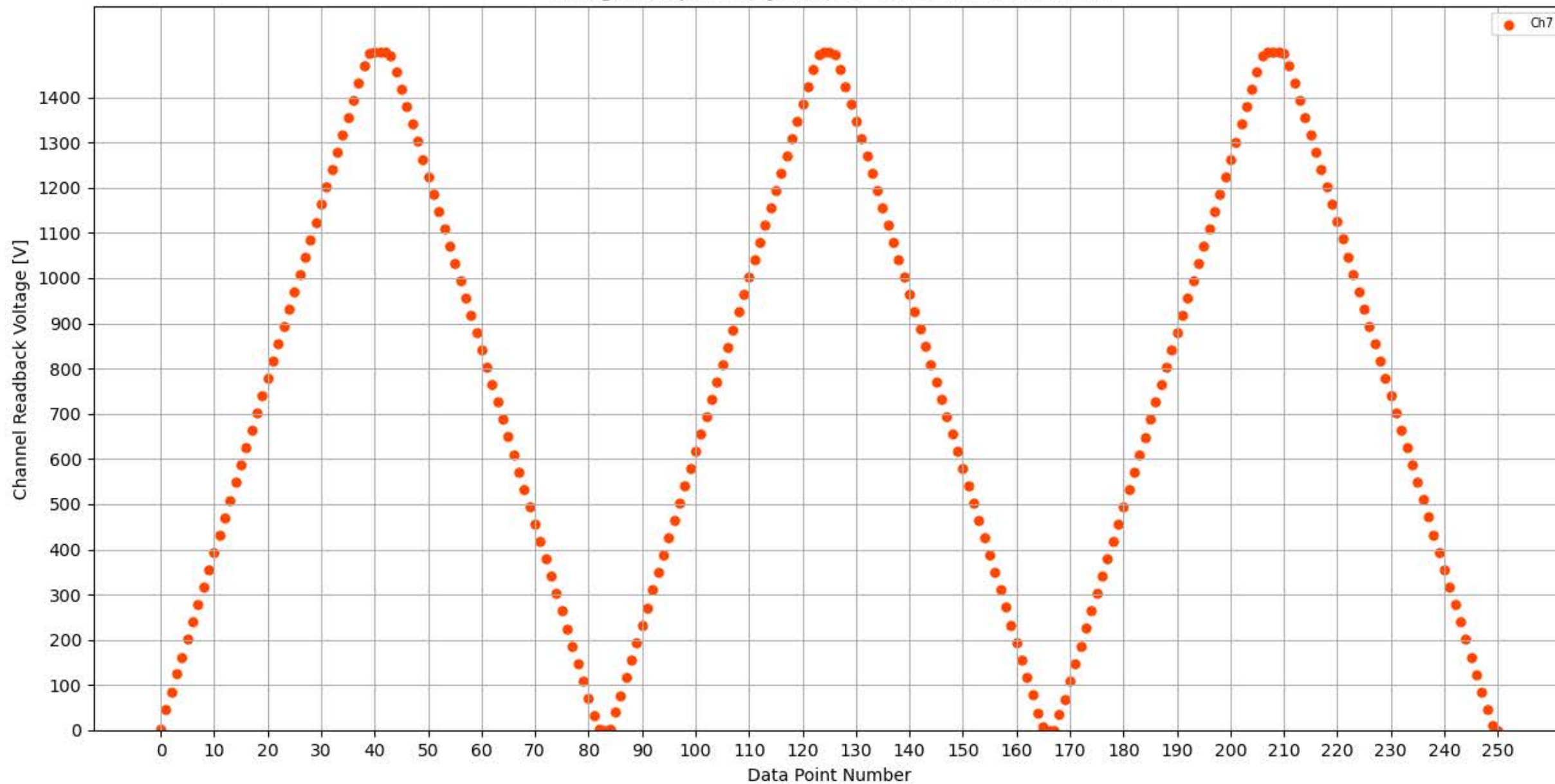
Voltage Ramp Test (Python) Bd #354, Slot #14, Ch #7
