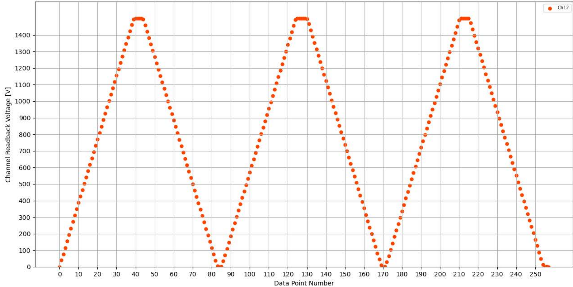
Voltage Ramp Test (Python) Bd #354, Slot #14, Ch #12
