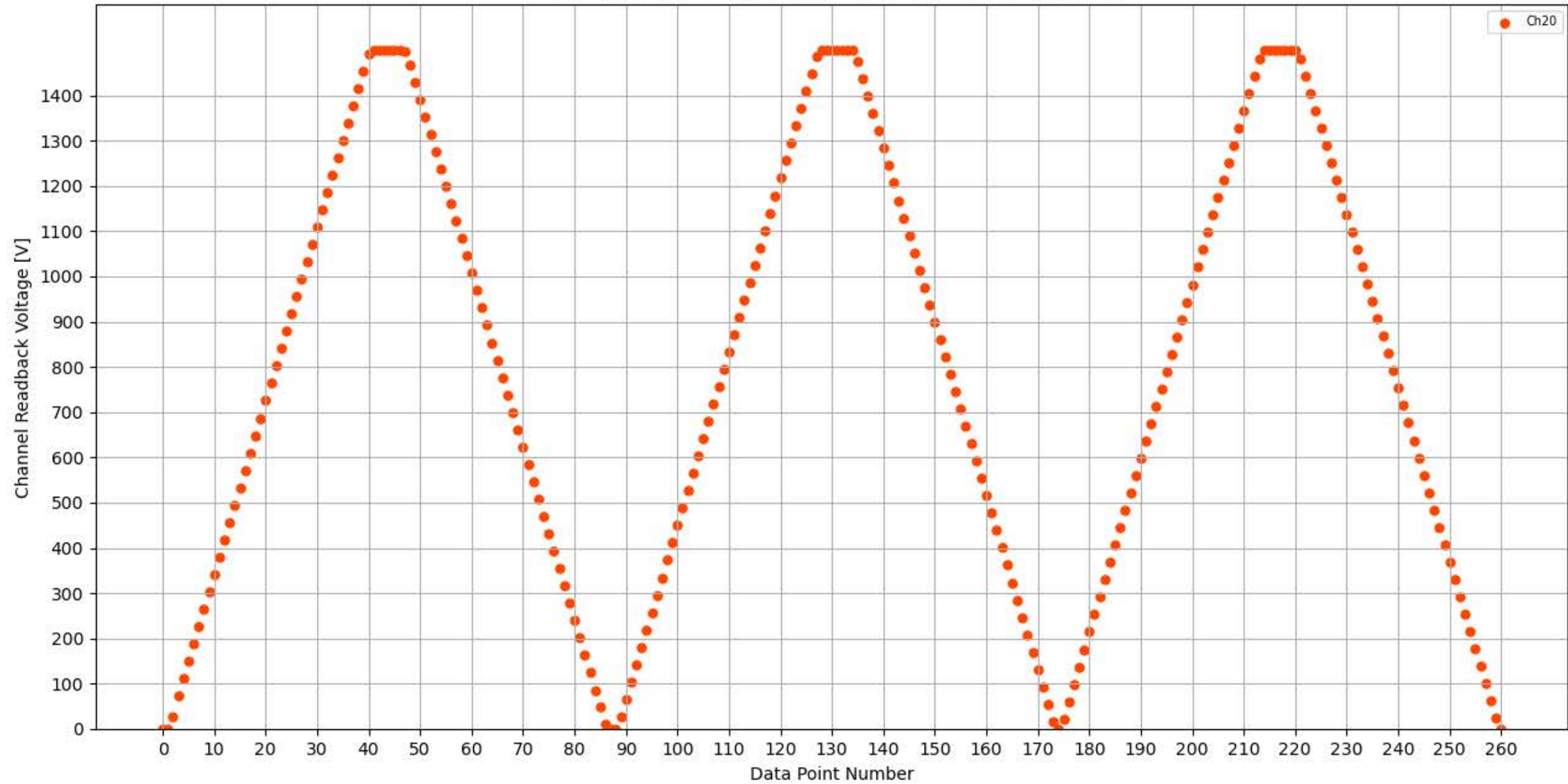
Voltage Ramp Test (Python) Bd #354, Slot #14, Ch #20
