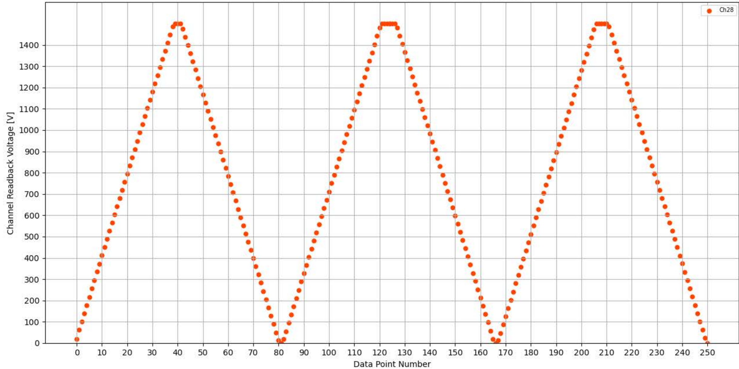
Voltage Ramp Test (Python) Bd #354, Slot #14, Ch #28
