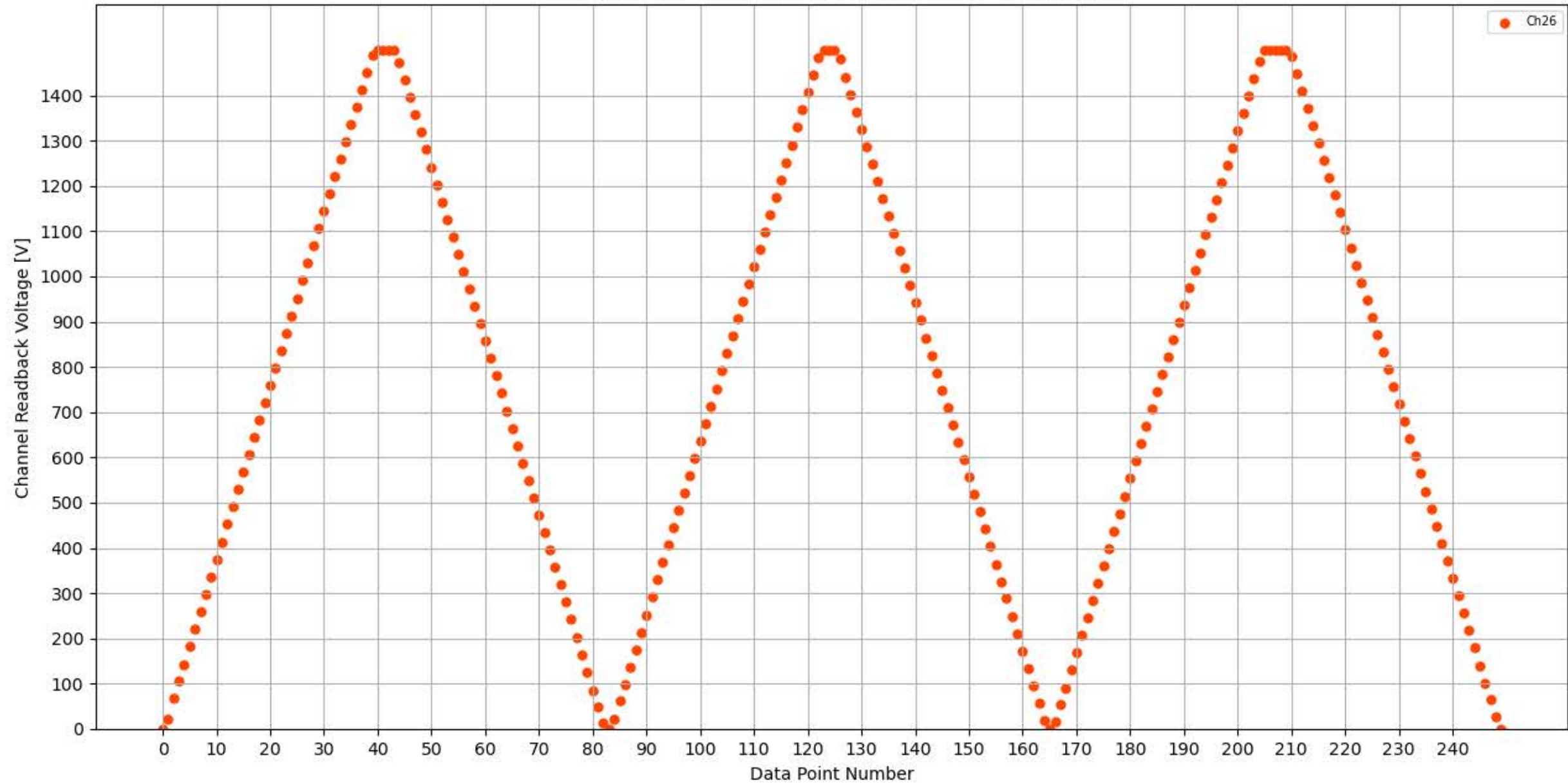
Voltage Ramp Test (Python) Bd #354, Slot #14, Ch #26
