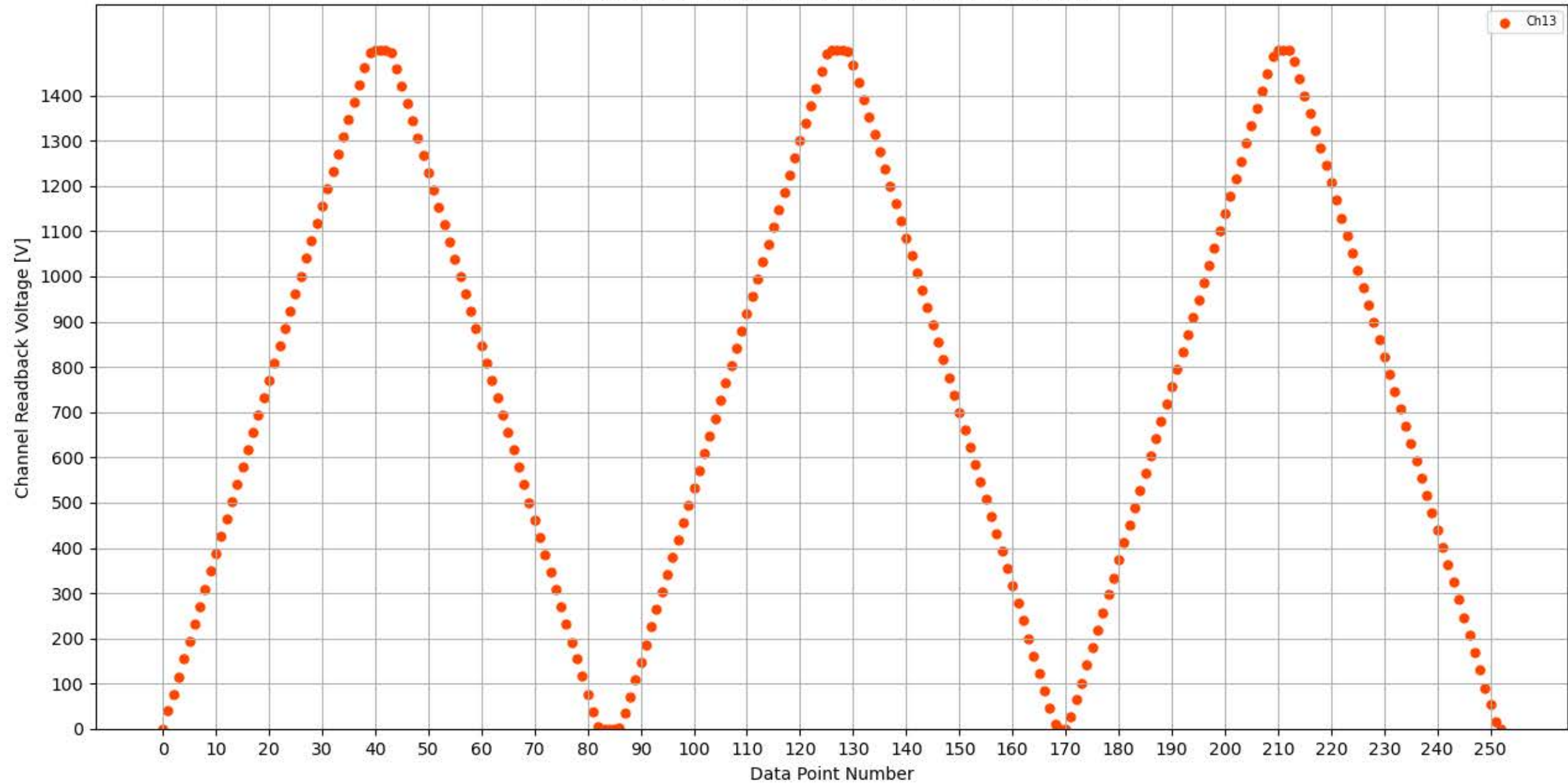
Voltage Ramp Test (Python) Bd #354, Slot #14, Ch #13
