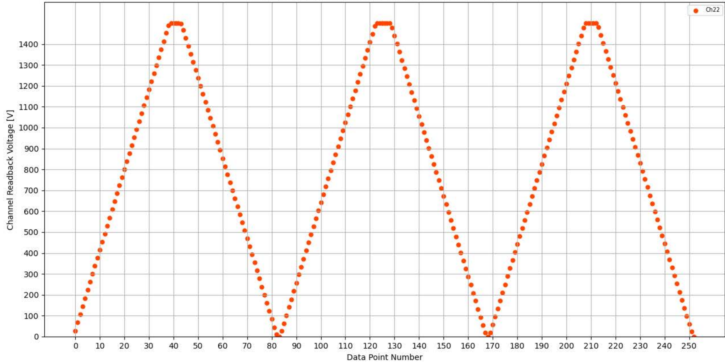
Voltage Ramp Test (Python) Bd #354, Slot #14, Ch #22
