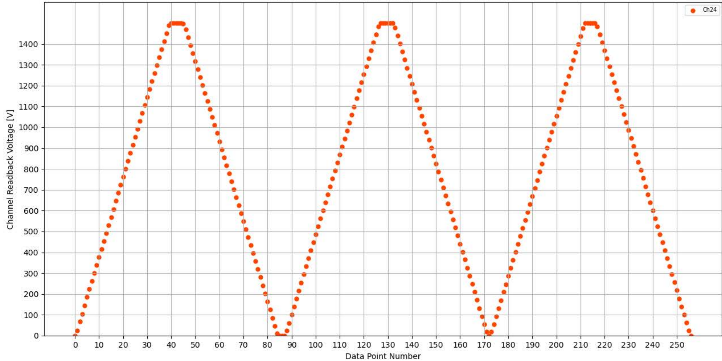
Voltage Ramp Test (Python) Bd #354, Slot #14, Ch #24
