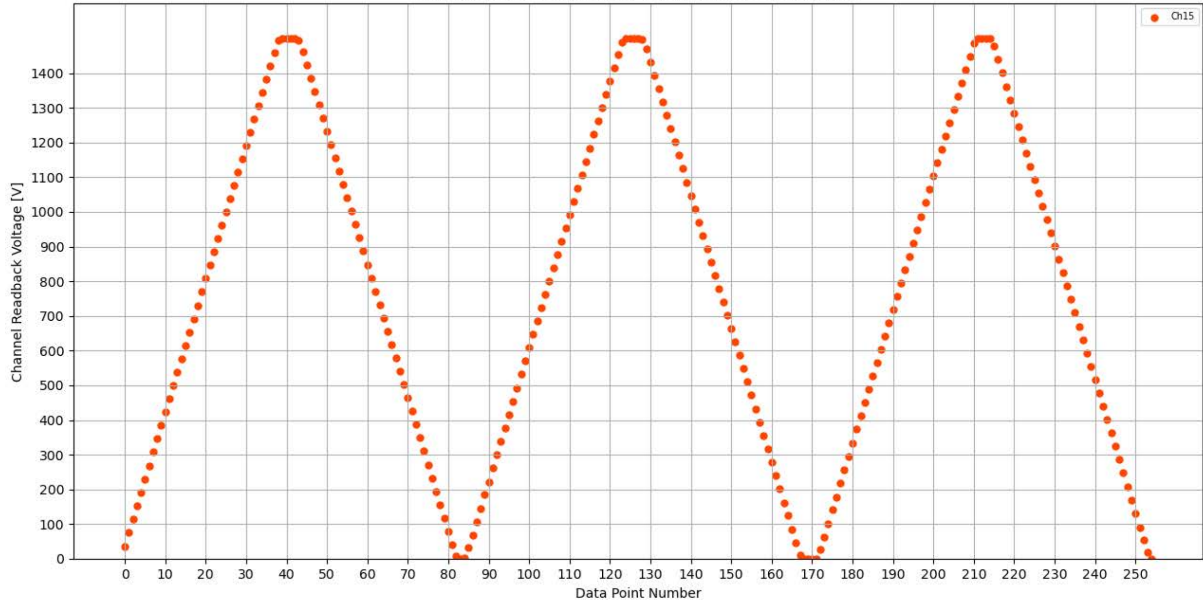
Voltage Ramp Test (Python) Bd #354, Slot #14, Ch #15
