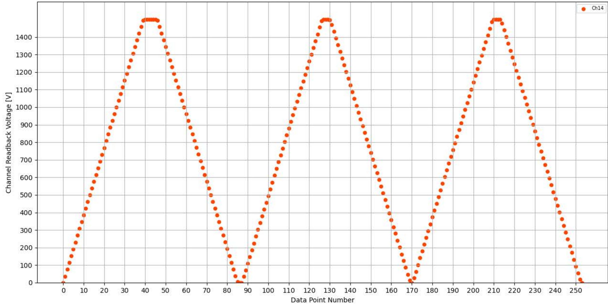
Voltage Ramp Test (Python) Bd #354, Slot #14, Ch #14
