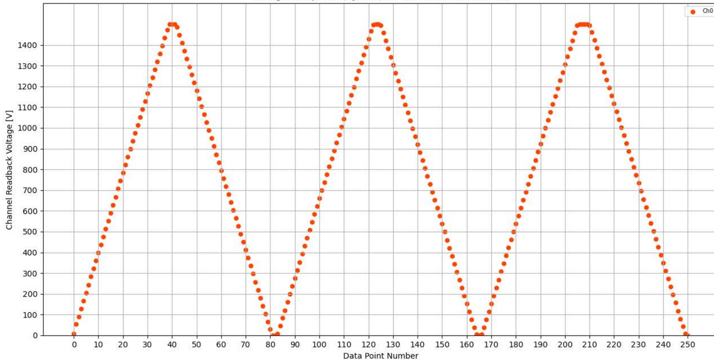
Voltage Ramp Test (Python) Bd #354, Slot #14, Ch #0
