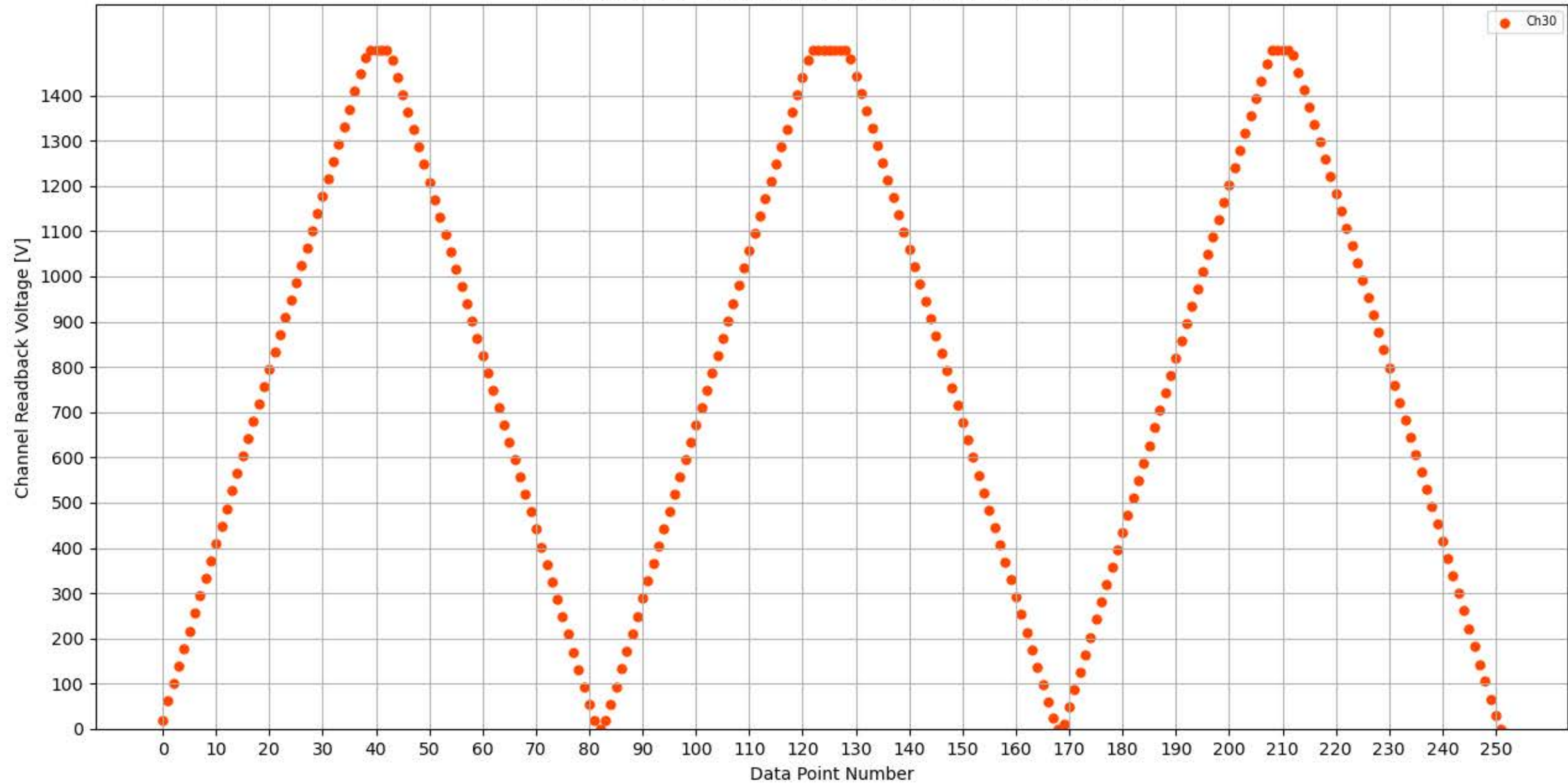
Voltage Ramp Test (Python) Bd #354, Slot #14, Ch #30
