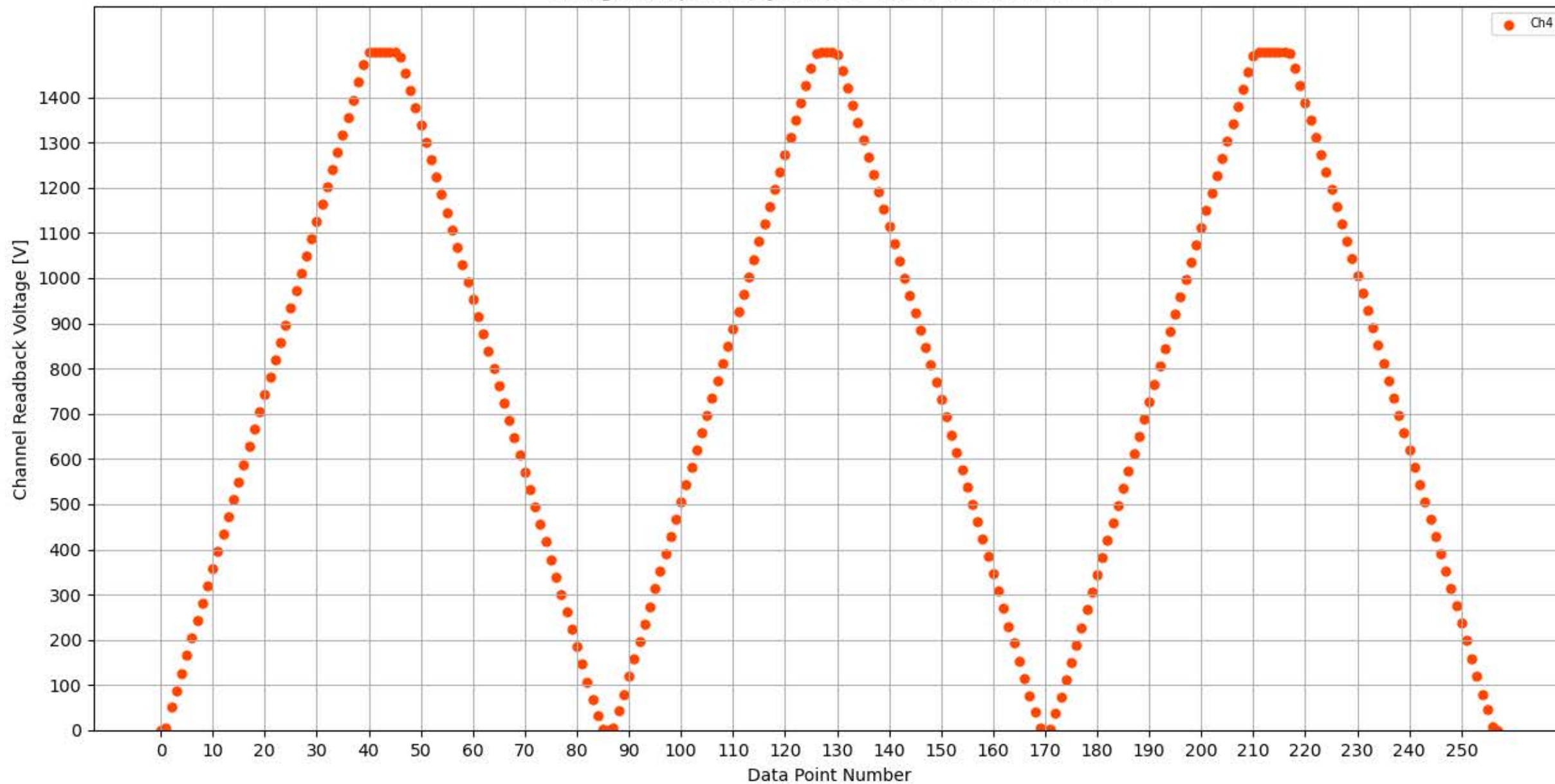
Voltage Ramp Test (Python) Bd #354, Slot #14, Ch #4
