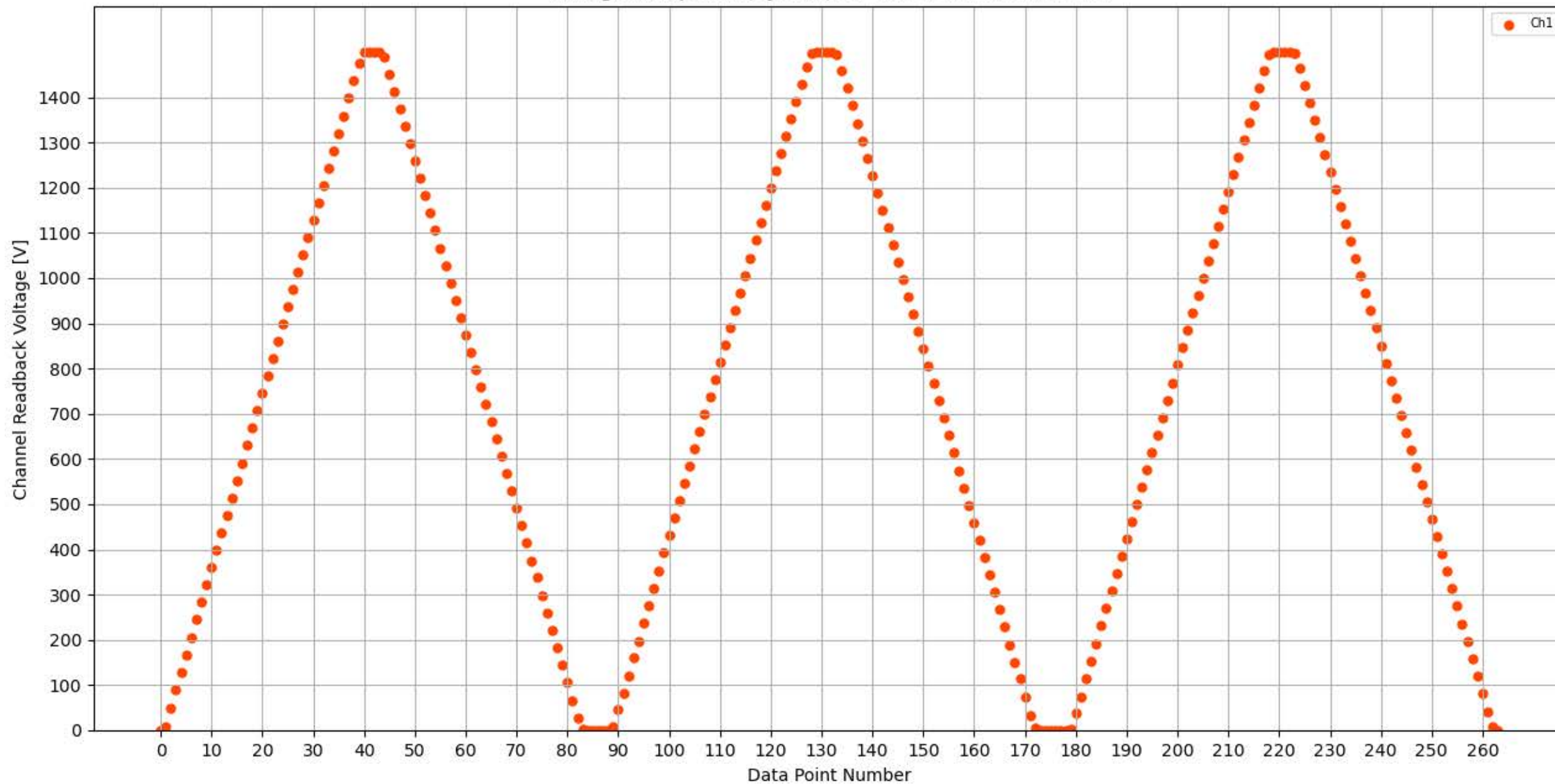
Voltage Ramp Test (Python) Bd #354, Slot #14, Ch #1
