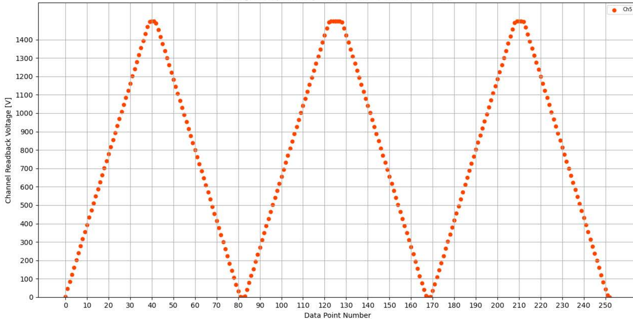
Voltage Ramp Test (Python) Bd #354, Slot #14, Ch #5
