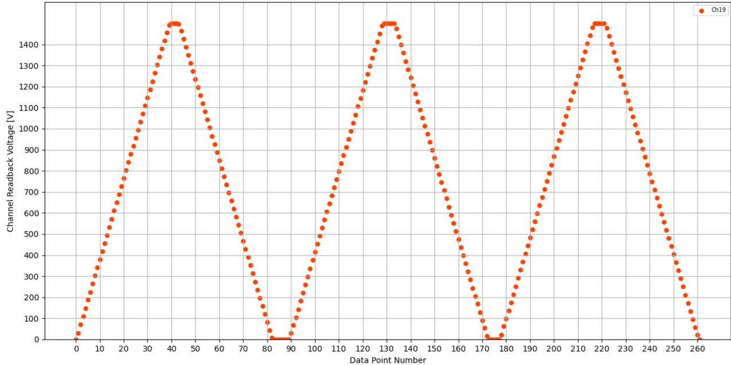
Voltage Ramp Test (Python) Bd #354, Slot #14, Ch #19
